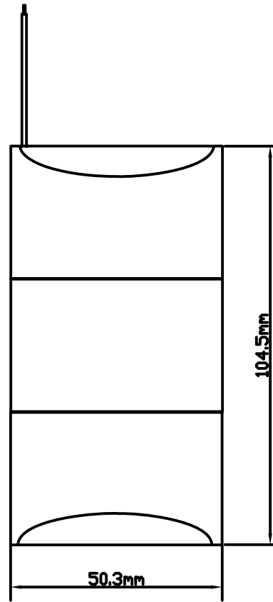
11.1V 1200mAh(3S1P)
